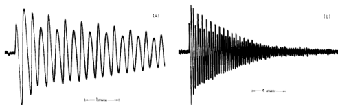
Figure 1: Experimental photocell current as a function of time after the field is switched to the x direction. Frequency of the 2\omega_p component is 4 kHz [23].
