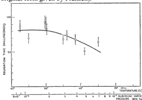
Figure 2: Variation of the relaxation time with the rubidium vapor pressure for an evacuated cell lined with tetracontane [26].
